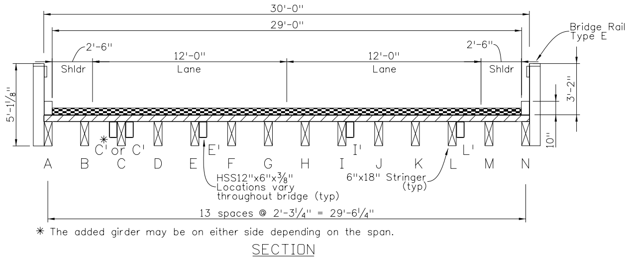
Fig. 1.13-4 Structure Component Naming Convention for Timber Sister Beams
